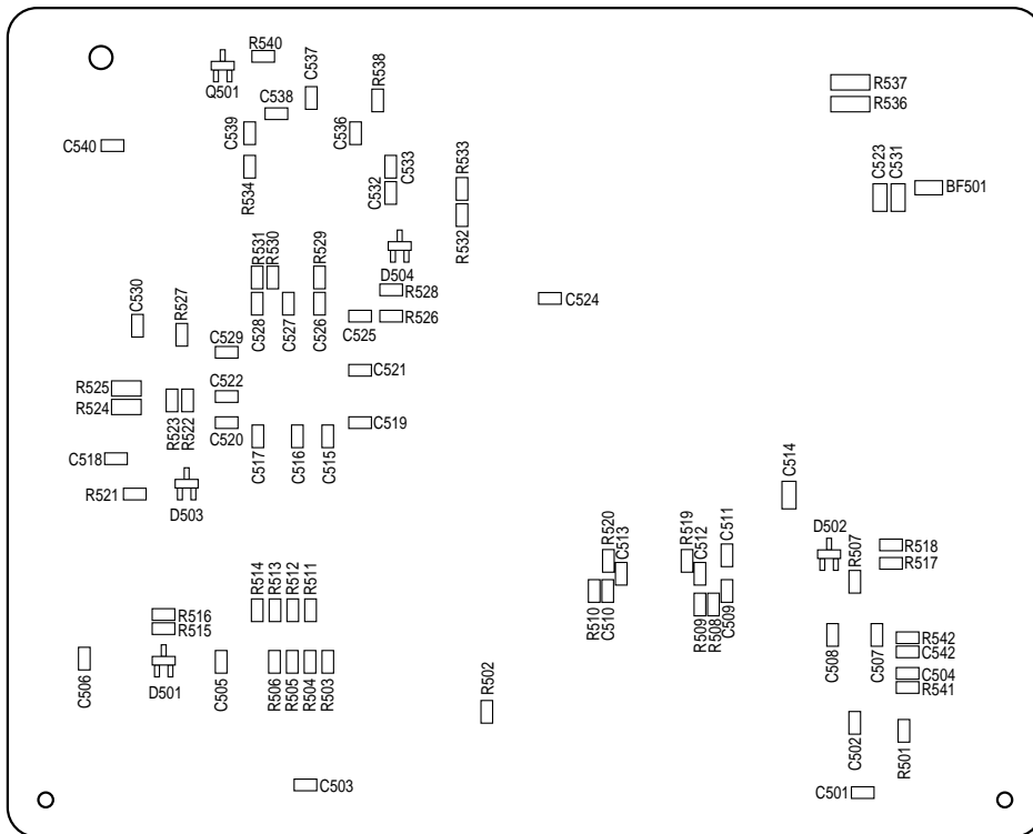
U8S Printed Circuit Board Rev.1 (41222702YA-1/2)
